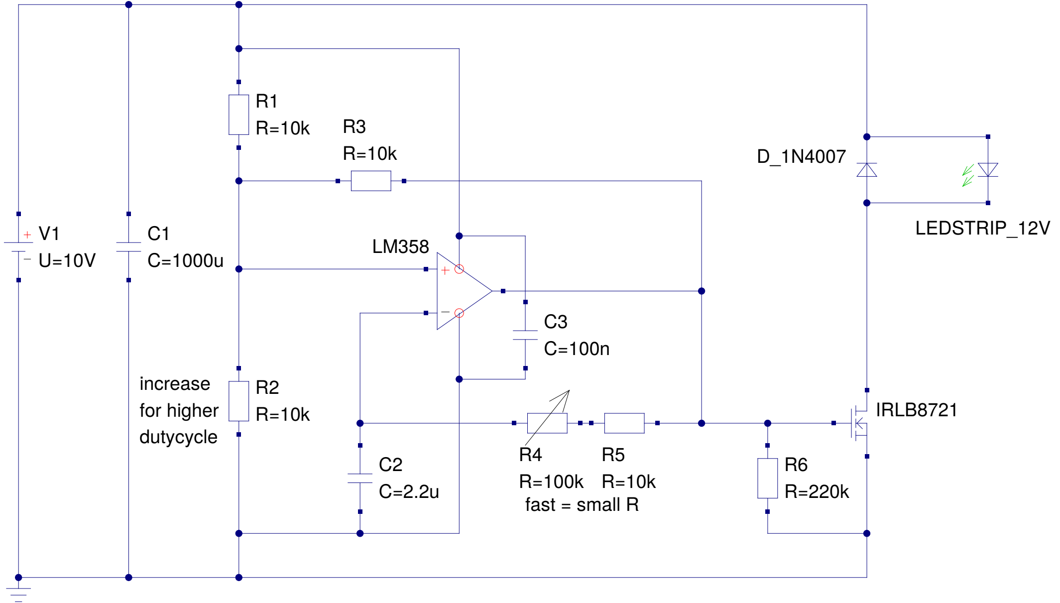
Opamp astable multivibrator (based on single-supply Schmitt-trigger circuit)
